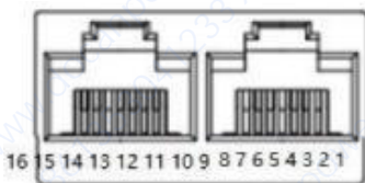
RS485
