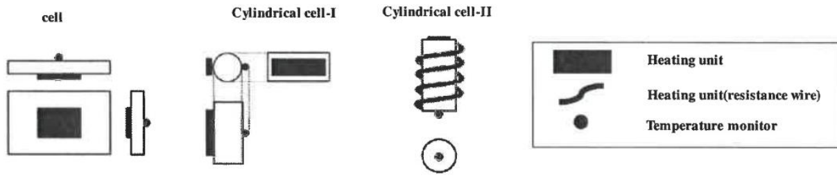
Fig.7 Schematic diagram of thermal runaway experiment
