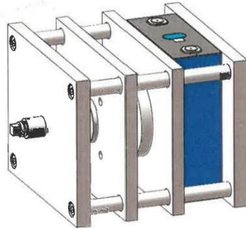
Fig.5 Diagram of cell with a swelling force clamp
