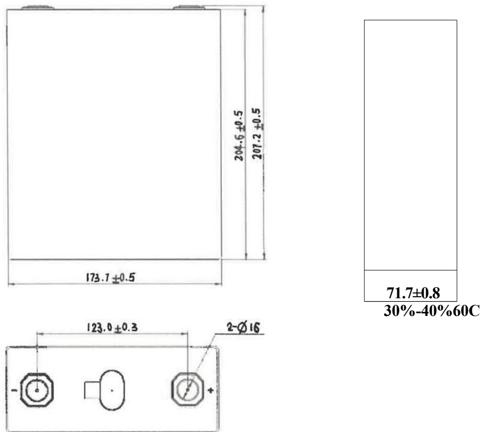
Fig.9 Diagram of cell size and appearance
